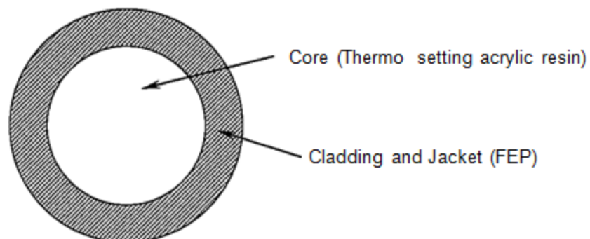
Fig.1 Cross-section of fiber
